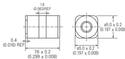
Surface-mount (GTCS35-XXXM-R05)
